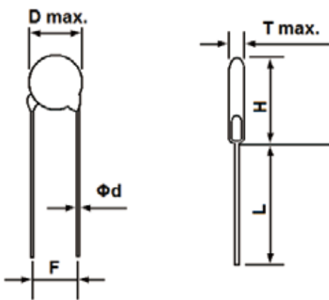
Kinked Lead (Y Type)
