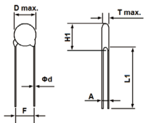
Straight Lead (P Type)
