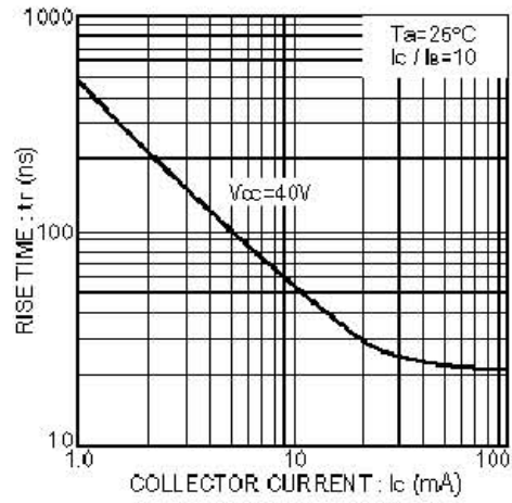
Fig.6 Rise time vs. collector current
