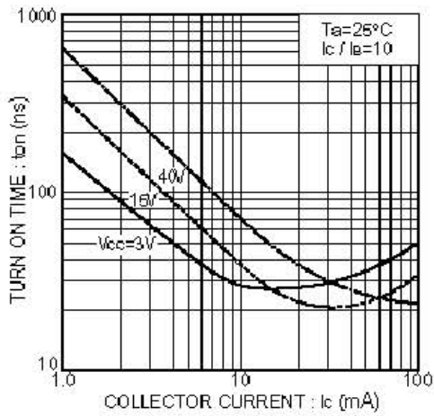
Fig.5 Turn-on time vs. collector current
