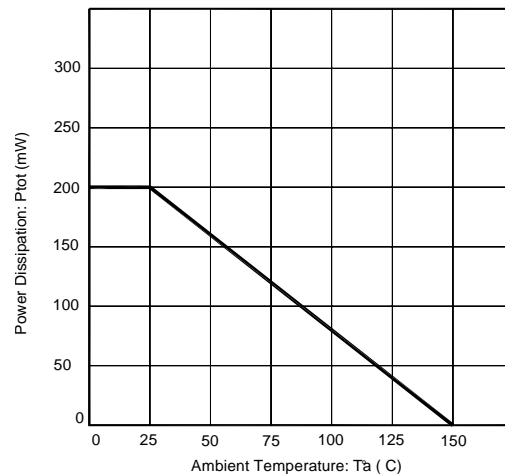
Fig.10 Power Dissipation vs Ambient Temperature
