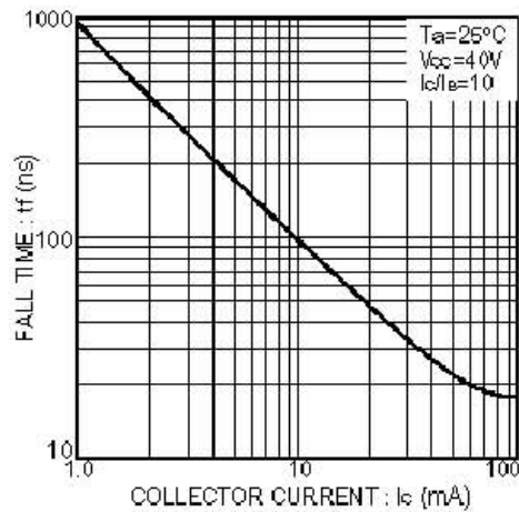
Fig.8 Fall time vs. collector current
